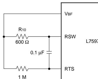
Figure 9. Ring Trip Threshold
