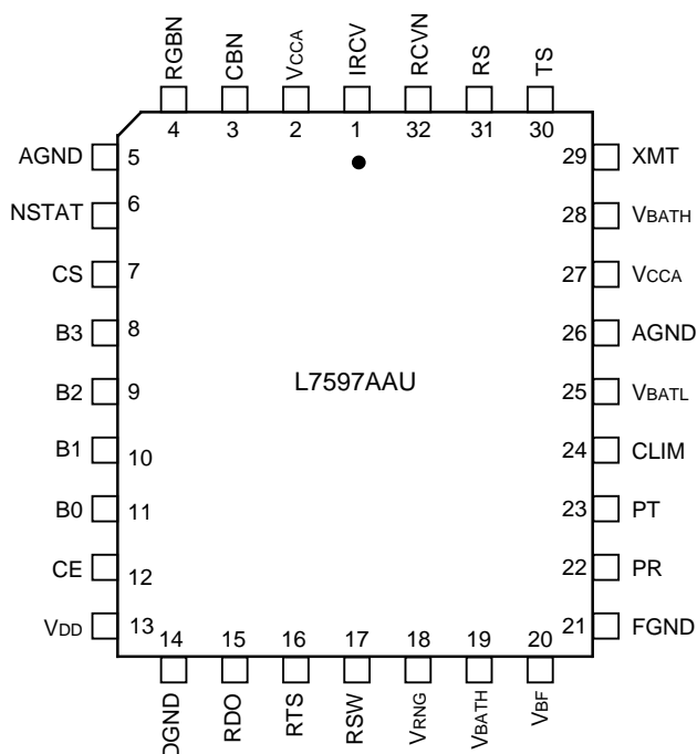
Figure 2. Pin Layout
