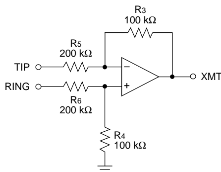
Figure 7. L7597 SLIC Matching Requirements
