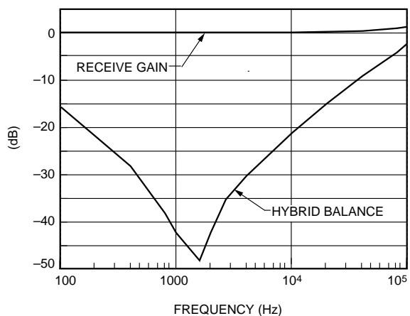
Figure 13. 7551 Receive Gain and Hybrid Balance vs. Frequency
