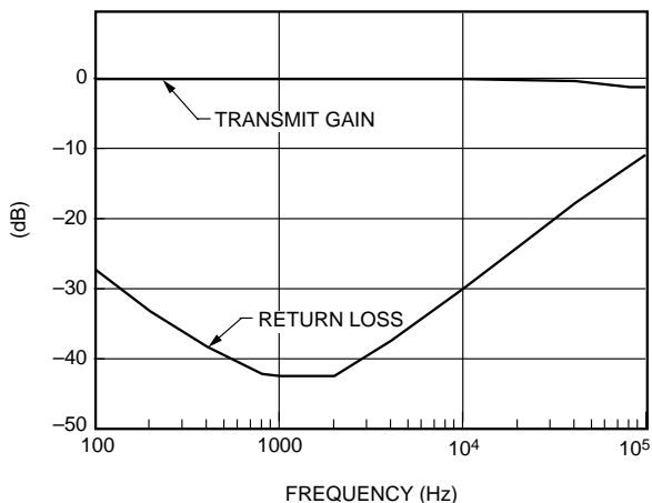
Figure 14. 7551 Transmit Gain and Return Loss vs. Frequency
