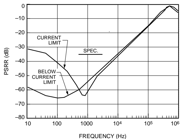
Figure 15. 7551 Typical V_{CC} Power Supply Rejection
