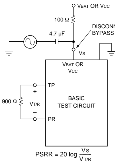
Figure 5. Metallic PSRR
