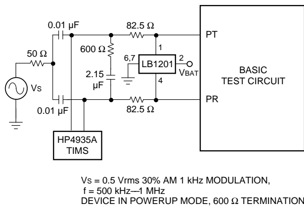
Figure 8. RFI Rejection
