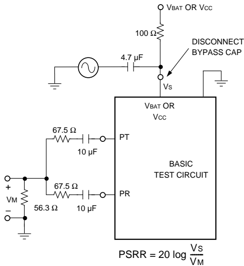
Figure 6. Longitudinal PSRR
