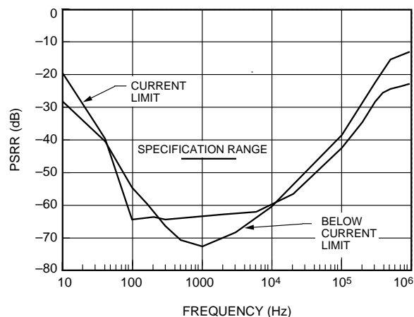
Figure 16. 7551 Typical V_{BAT} Power Supply Rejection
