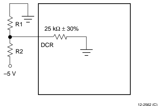
Figure 27. Equivalent Circuit for Adjusting the Overhead Voltage
