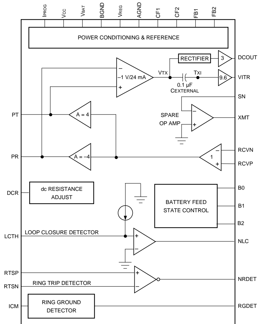
Figure 1. Functional Diagram
