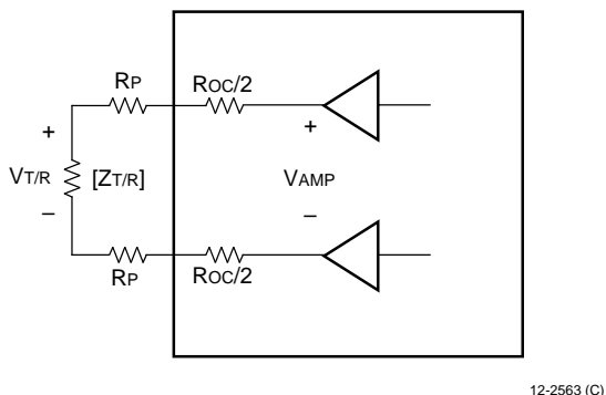
Figure 26. SLIC 2-Wire Output Stage
