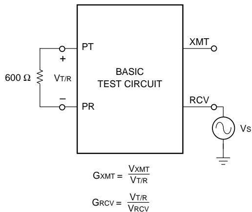
Figure 10. ac Gains
