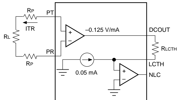
Figure 30. Off-Hook Detection Circuit
