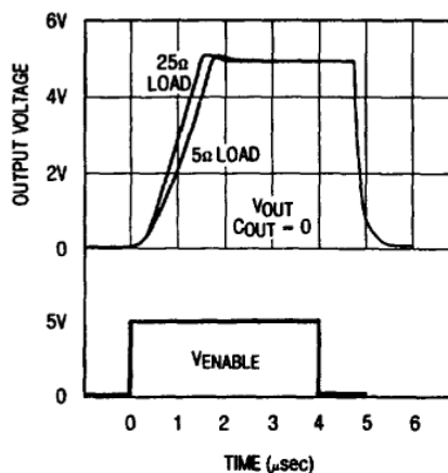
Switching Characteristics
