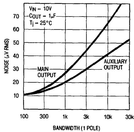
Output Noise
