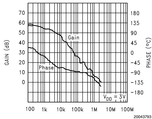
Open Loop Frequency Response, 3V
