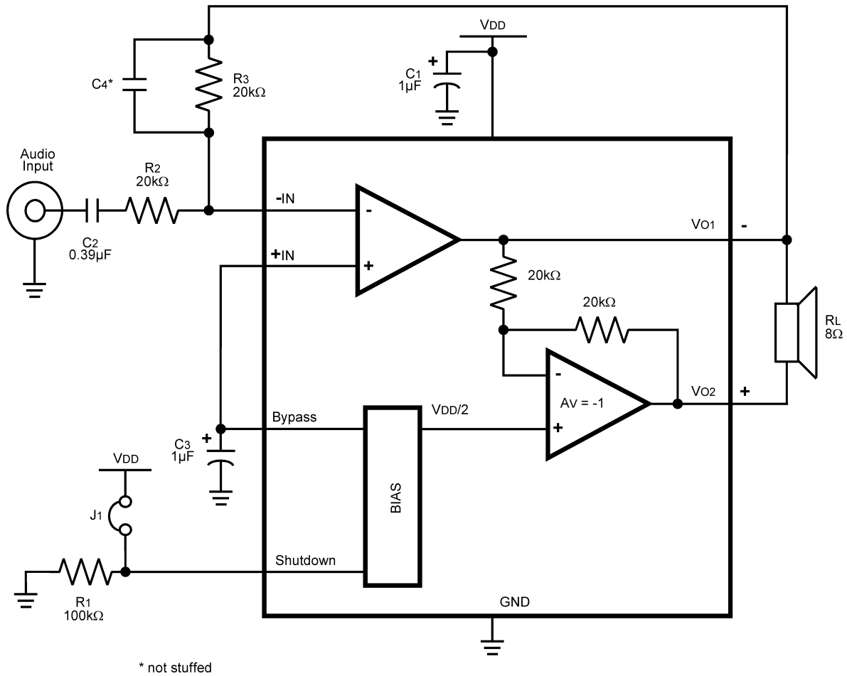
FIGURE 4. REFERENCE DESIGN BOARD SCHEMATIC
