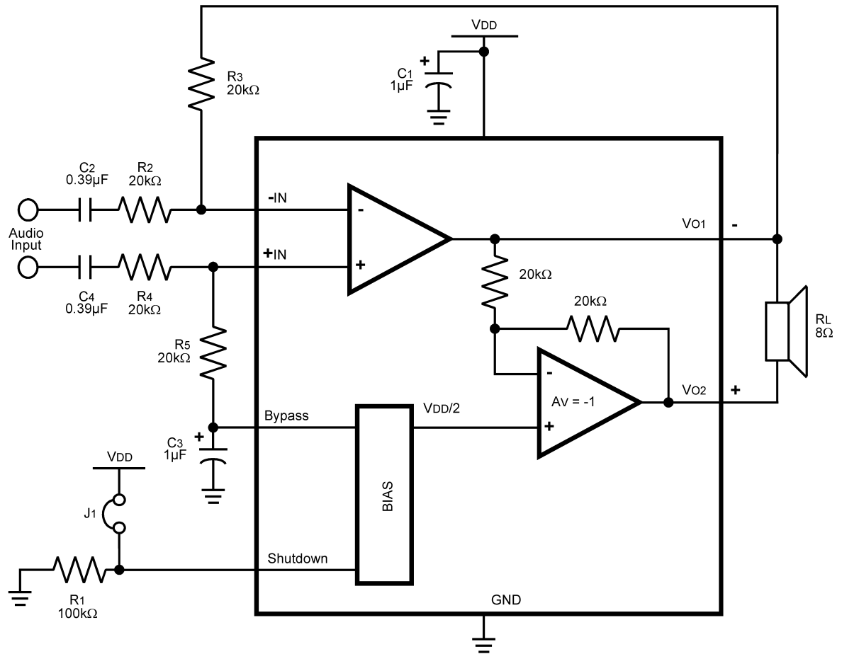
FIGURE 3. DIFFERENTIAL AMPLIFIER CONFIGURATION FOR LM4904
