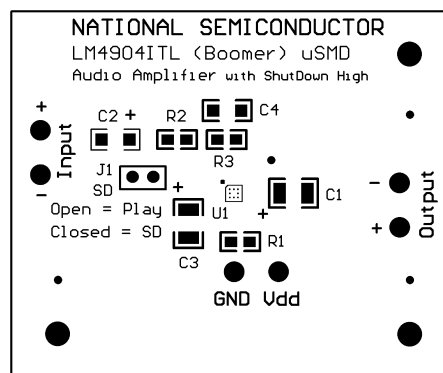
Silk Screen
