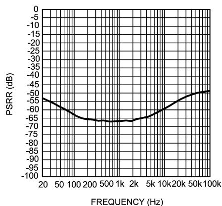
Power Supply Rejection Ratio V_{DD} = 1.5V , V_{RIPPLE} = 200mV_{PP} R_L = 8\Omega , BTL Input Terminated into 10\Omega
