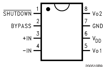
Top View Order Number LM4990MM See NS Package Number MUA08A
