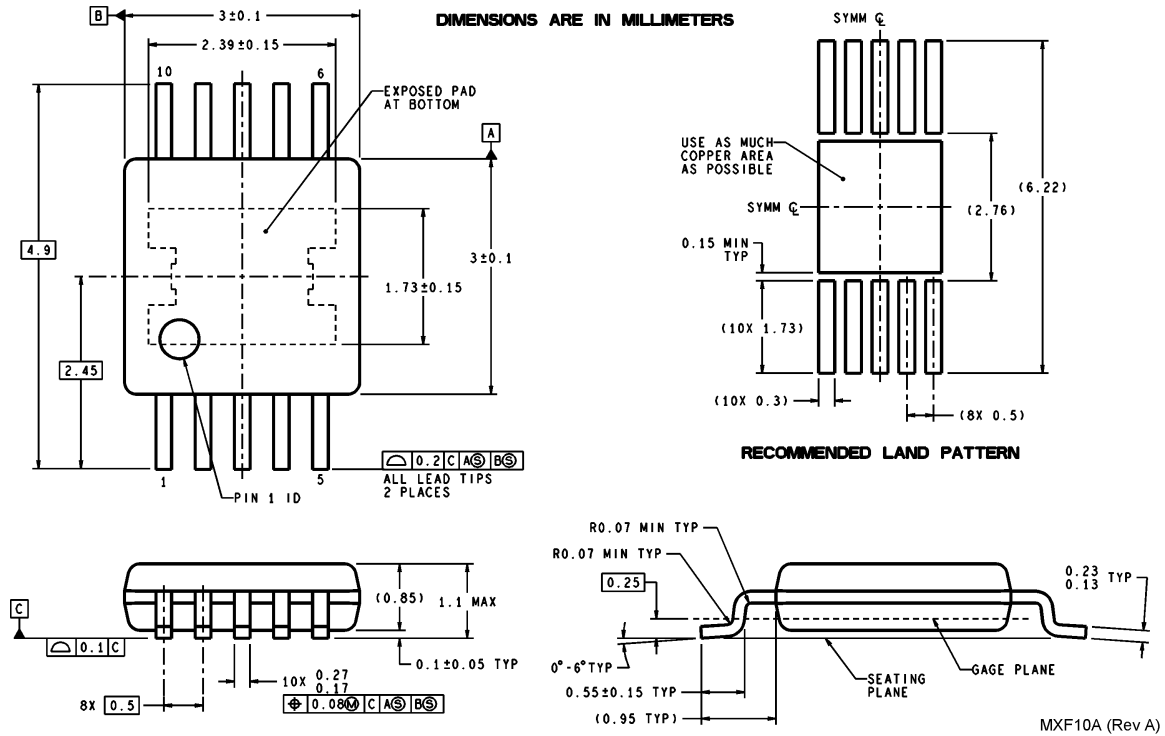
Exposed-DAP TSSOP Order Number LM4990MH NS Package Number MXF10A
