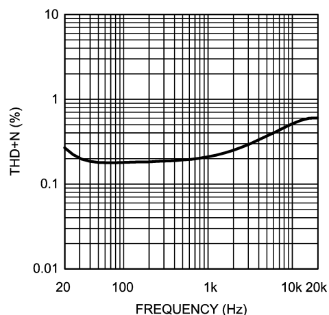
THD+N vs Frequency V_{DD} = 3V , R_L = 4\Omega , and P_O = 500mW
