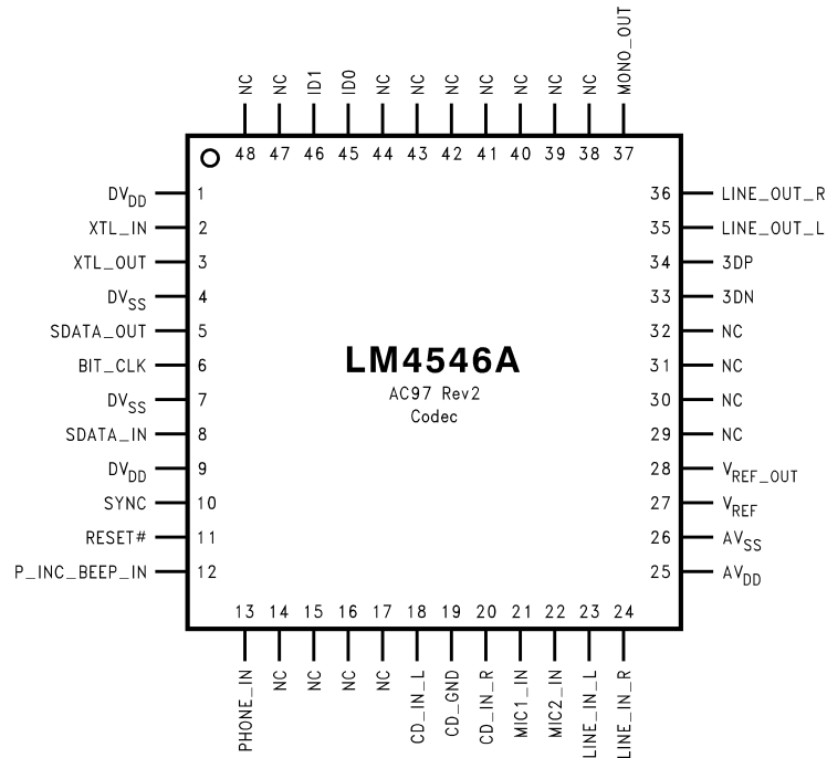
Top View Order Number LM4546AVH See NS Package Number VBH48A
