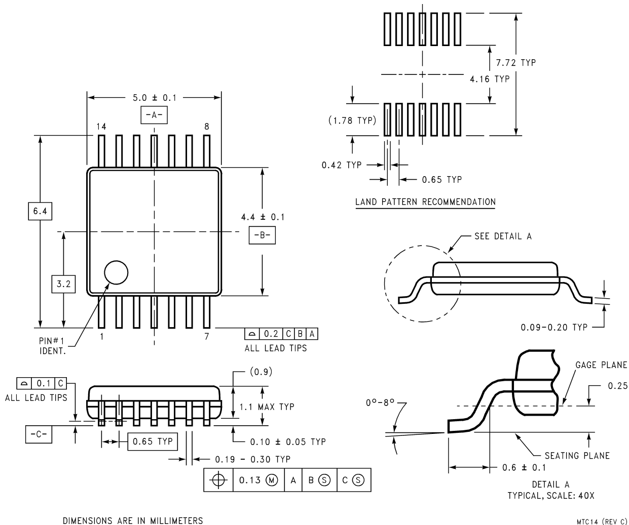
14-Pin TSSOP NS Package Number MTC14
