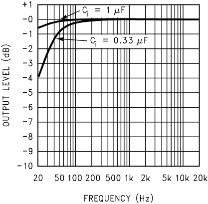
Frequency Response vs Input Capacitor Size
