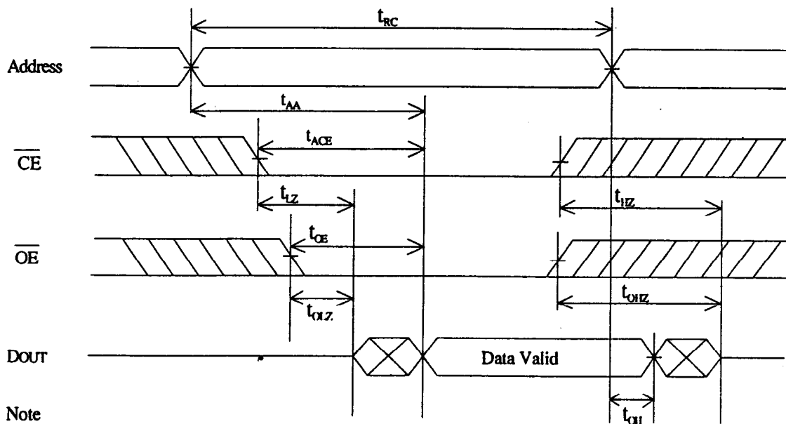
Read cycle timing chart (*7)
