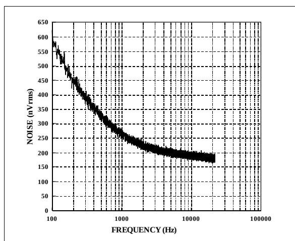
Figure 8 : Noise vs Frequency ( I_{\text{LOAD max}} - V_{\text{IN min}} )
