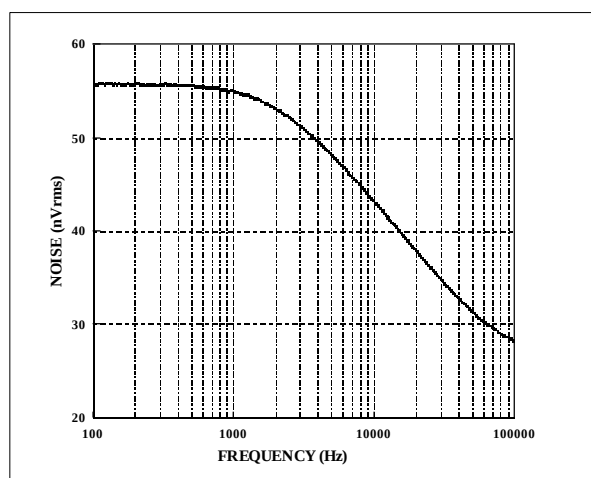
Figure 7 : PSRR vs Frequency ( I_{\text{LOAD max}} - V_{\text{IN min}} )
