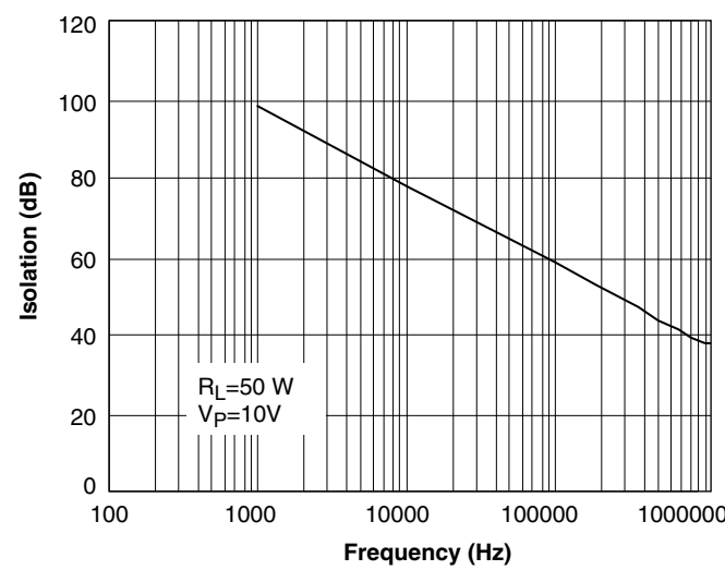
Figure 11. Output Isolation
