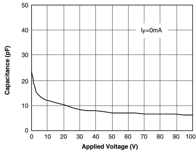
Figure 10. Switch Capacitance vs. Applied Voltage
