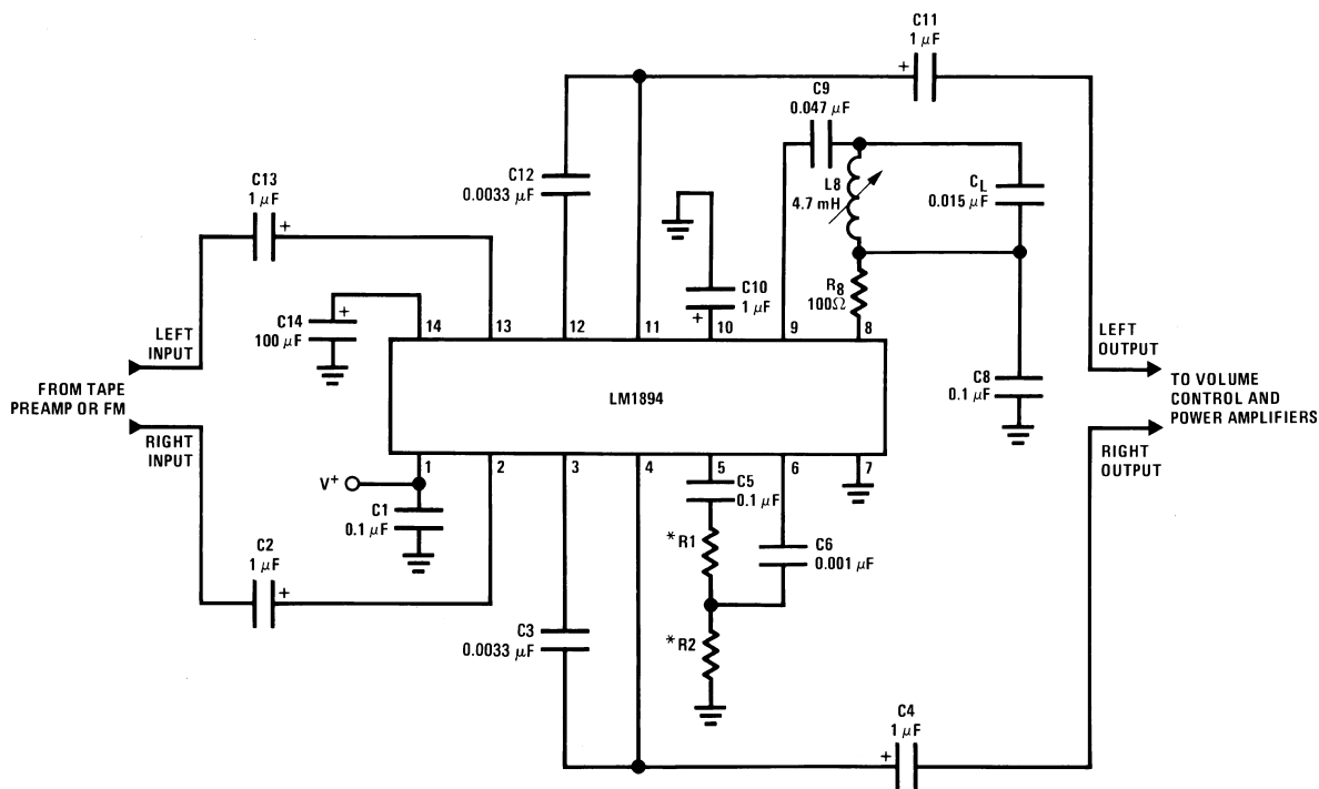
Order Number LM1894M, LM1894N, or LM1894MT See NS Package Number M14A, N14A, or MTC14 FIGURE 1. Component Hook-Up for Stereo DNR System
