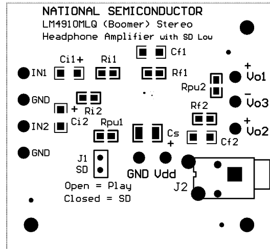
Silk Screen
