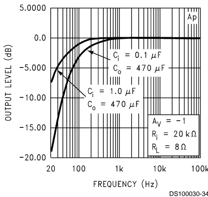
Typical Application Frequency Response
