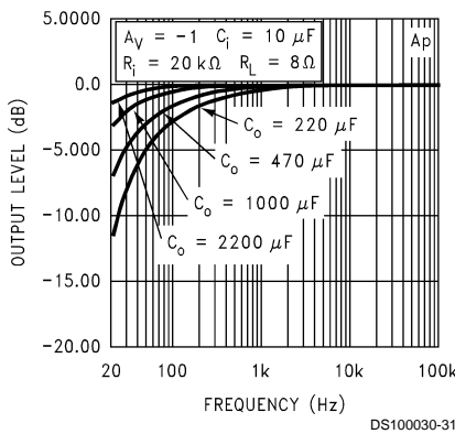
Frequency Response vs Output Capacitor Size
