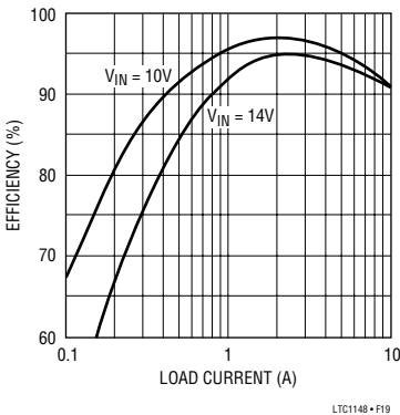
Figure 19. All N-Channel 5V/8A Efficiency
