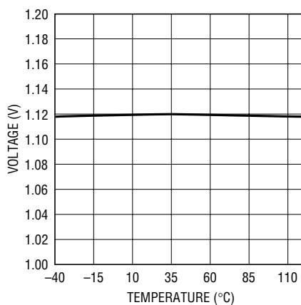
PGFB Threshold
