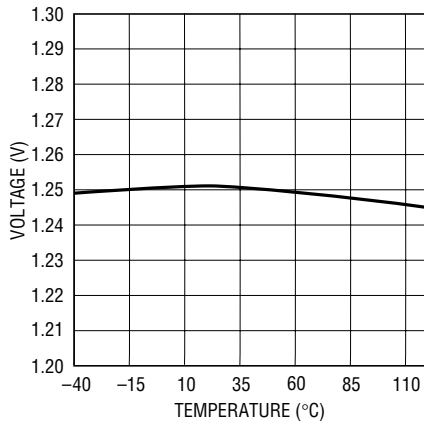
FB Voltage
