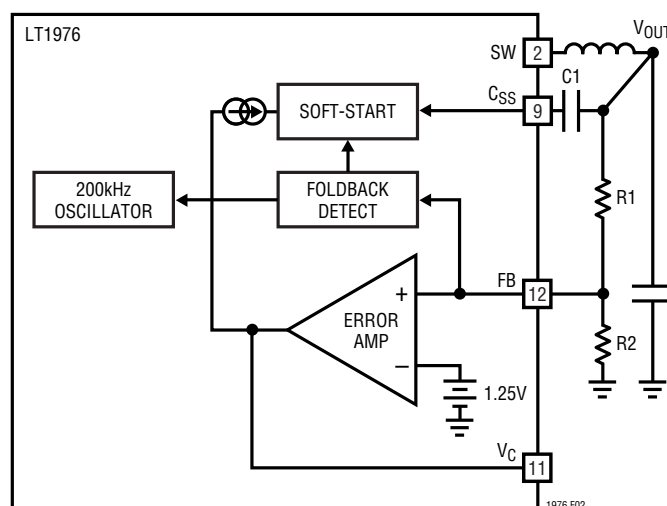
Figure 2. Feedback Network
