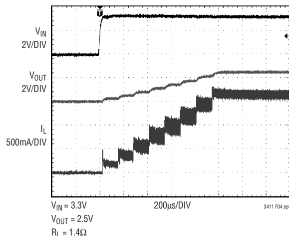
Figure 4. Digital Soft-Start
