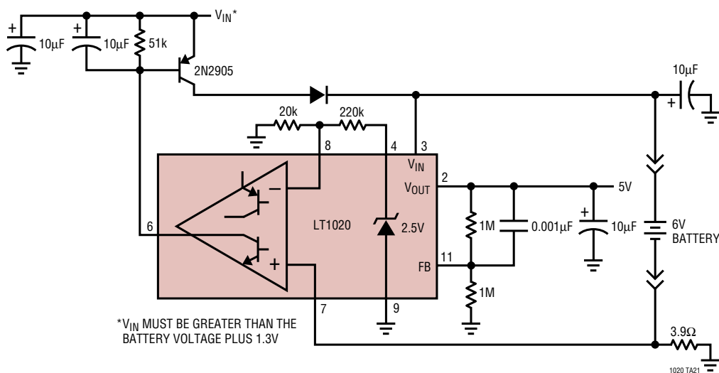
Switching Preregulator for Wide Input Voltage Range
