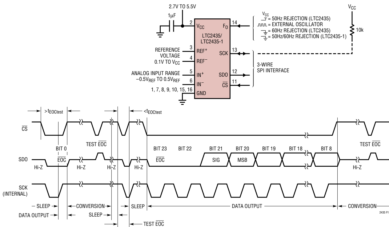
Figure 12. Internal Serial Clock, Reduced Data Output Length
