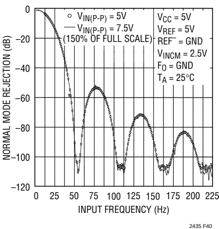
Figure 40. Measured Input Normal Mode Rejection vs Input Frequency ( f_N = 54.6Hz )
