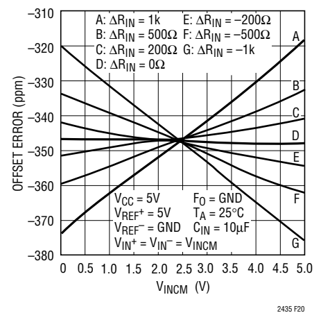
Figure 20. Offset Error vs Common Mode Voltage ( V_{INCM} = V_{IN^+} = V_{IN^-} ) and Input Source Resistance Imbalance ( \Delta R_{IN} = R_{SOURCEIN^+} - R_{SOURCEIN^-} ) for Large C_{IN} Values ( C_{IN} \geq 1\mu F )
