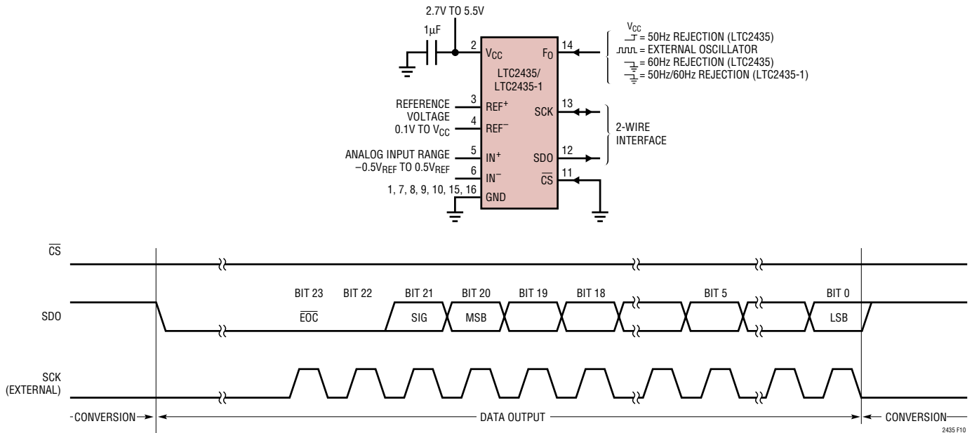
Figure 10. External Serial Clock, \overline{\text{CS}} = 0 Operation (2-Wire)
