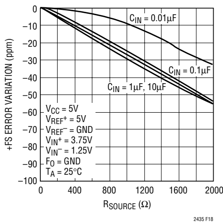
Figure 18. +FS Error vs R_{SOURCE} at IN^+ or IN^- (Large C_{IN} )
