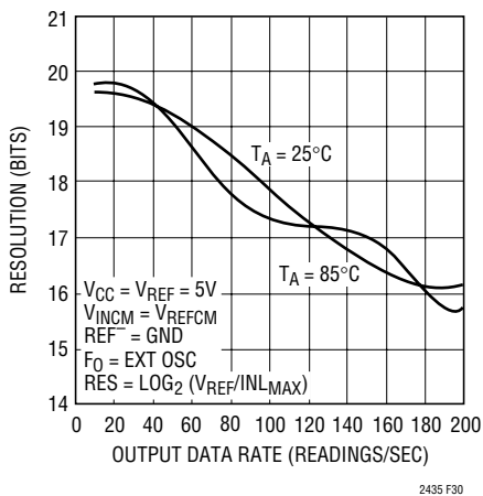
Figure 30. Resolution ( \text{INL}_{\text{RMS}} \leq 1\text{LSB} ) vs Output Data Rate and Temperature
