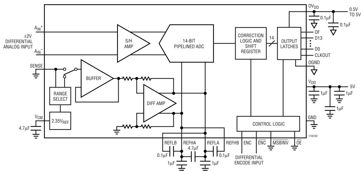
80Mps, 14-Bit ADC with a 2V Differential Input Range
