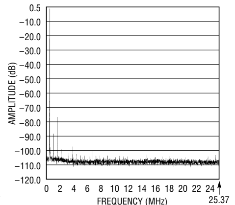
Averaged, 8192 Point FFT, Input Frequency = 51MHz, -1dB, 2V Range
