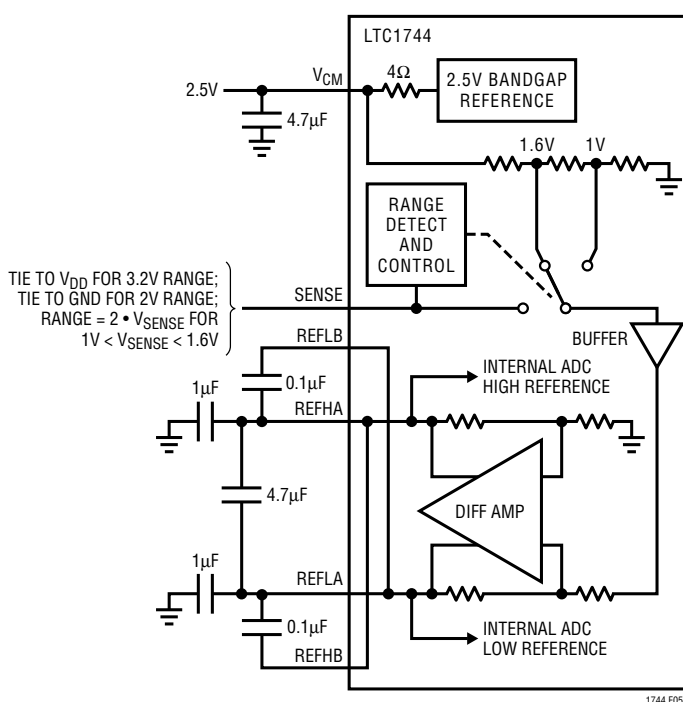
Figure 5. Reference Circuit
