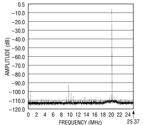
Averaged, 8192 Point FFT, Input Frequency = 20MHz, -6dB, 3.2V Range
