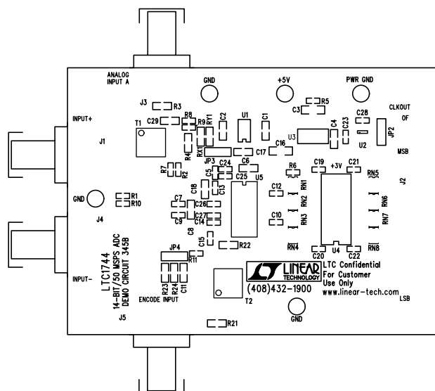
Topside Silkscreen
