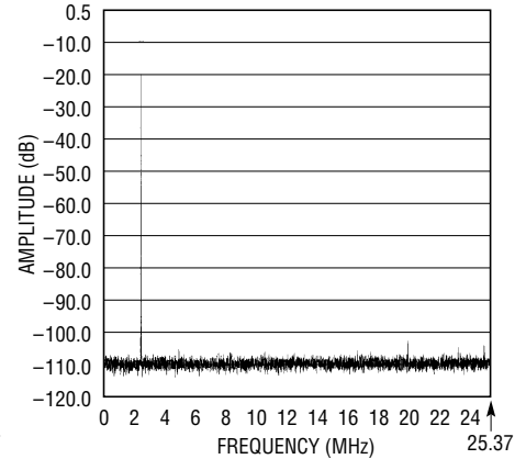
Averaged, 8192 Point FFT, Input Frequency = 2.5MHz, -20dB, 2V Range
