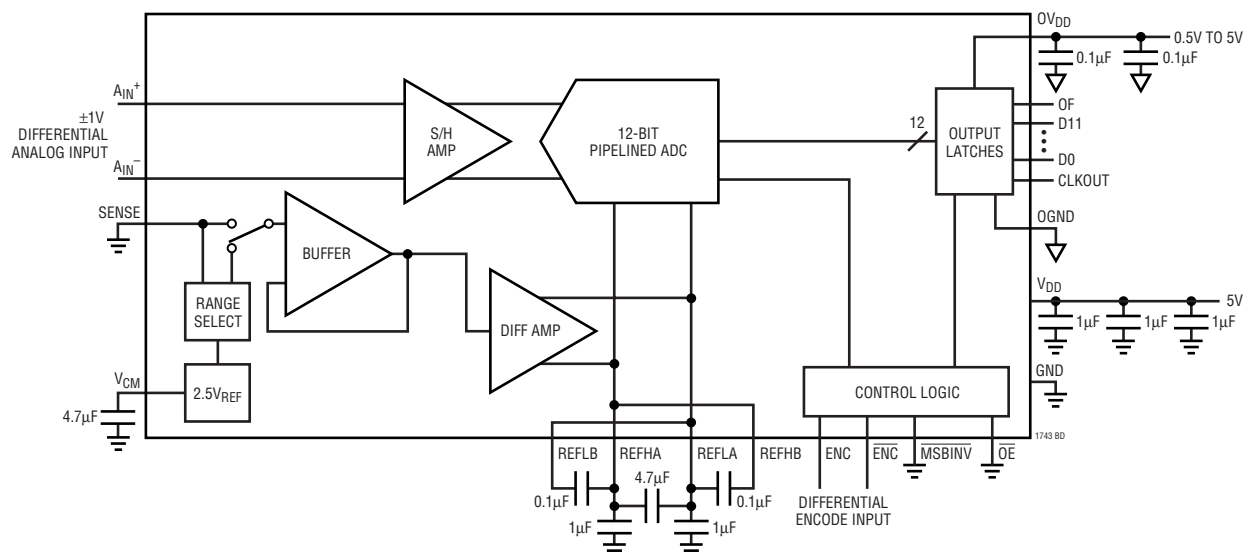
50Msps, 12-Bit ADC with a \pm 1V Differential Input Range
