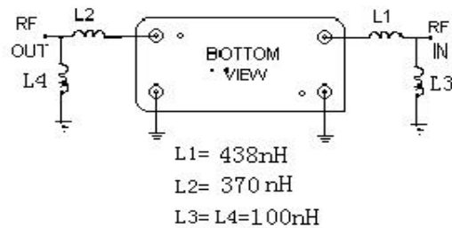
Matching configuration
