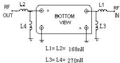
Matching configuration
