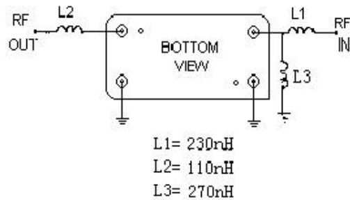
Matching configuration
