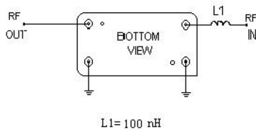
Matching configuration
