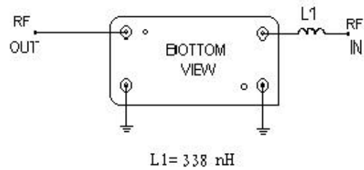
Matching configuration
