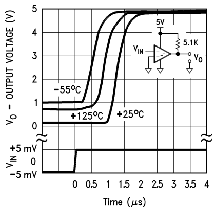
Comparator Response Times—Non-Inverting Input, Positive Transition
