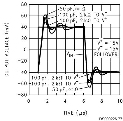
Small-Signal Pulse Response vs Load
