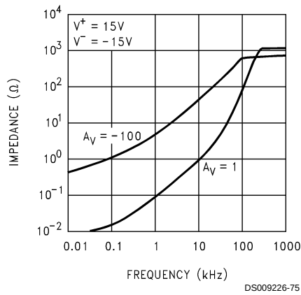
Output Impedance vs Frequency and Gain
