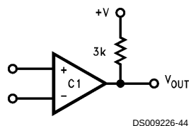
FIGURE 15. Basic Comparator
