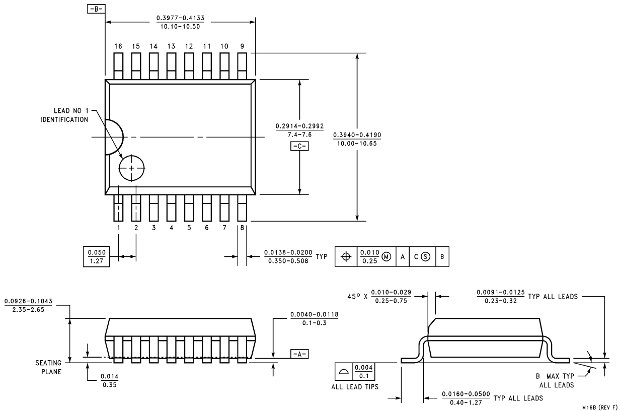
16-Lead Small Outline Package (WM) Order Number LM613IWM or LM613IWMX NS Package Number M16B
