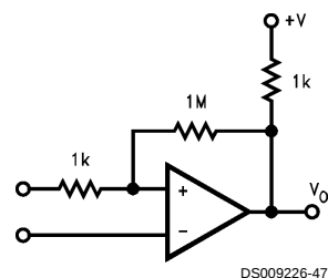
FIGURE 18. Comparator with Hysteresis ( \Delta V_H = +V(1k/1M) )
