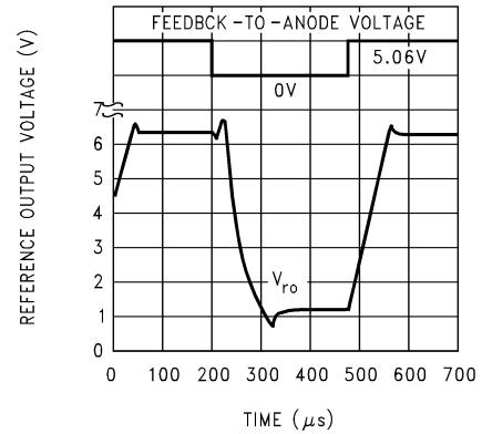
Reference Voltage with FEEDBACK Voltage Step
