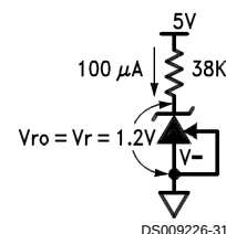
FIGURE 3. 1.2V Reference
