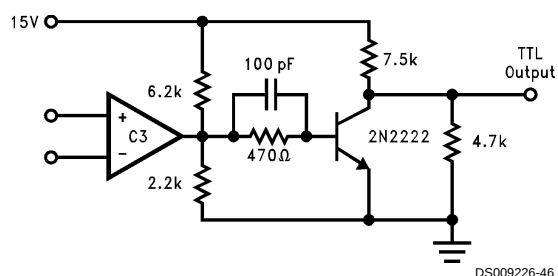
FIGURE 17. Wide-Input Range Comparator with TTL Output
