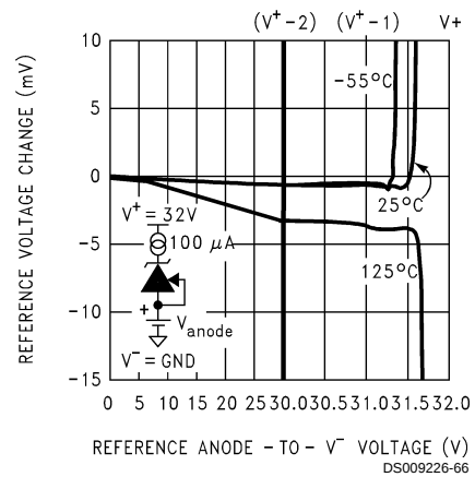
Reference Change vs Common-Mode Voltage
