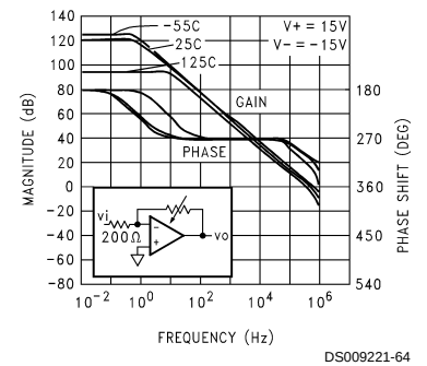
Small-Signal Voltage Gain vs Frequency and Temperature
