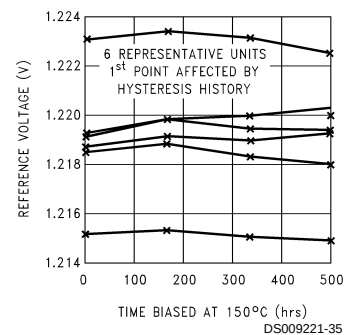
Accelerated Reference Voltage Drift vs Time
