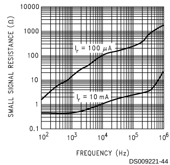
Reference Small-Signal Resistance vs Frequency
