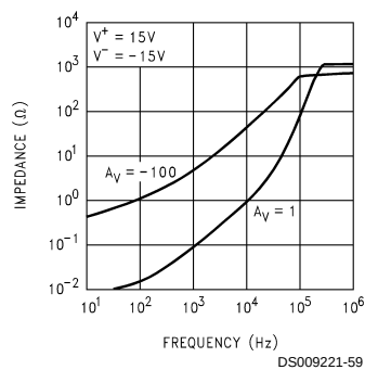
Output Impedance vs Frequency and Gain
