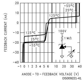
Feedback Current vs Feedback-to-Anode Voltage
