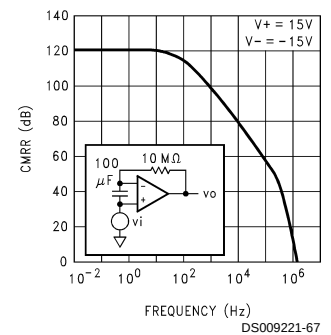
Common-Mode Input Voltage Rejection Ratio
