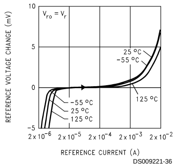
Reference Voltage vs Current and Temperature
