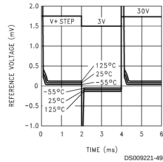
Reference Voltage Change with Supply Voltage Step
