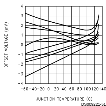
V_{OS} vs Junction Temperature
