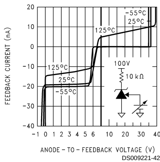
Feedback Current vs Feedback-to-Anode Voltage
