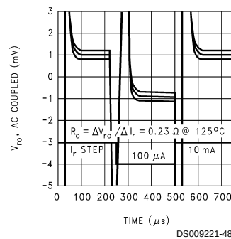
Reference Step Response for 100 \mu\text{A} ~ 10 mA Current Step
