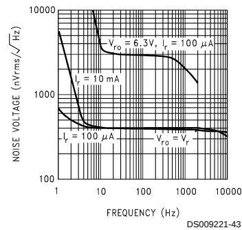
Reference Noise Voltage vs Frequency
