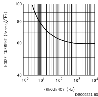
Op Amp Current Noise vs Frequency
