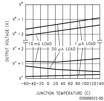
Output Voltage Swing vs Temp. and Current
