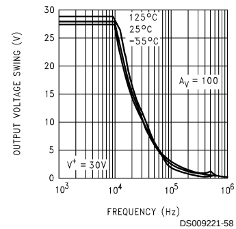
Output Swing, Large Signal
