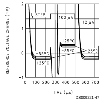
Reference Voltage with 100–12 \mu\text{A} Current Step
