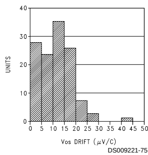
Average V_{OS} Drift Industrial Temperature Range
