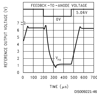
Reference Voltage with Feedback Voltage Step
