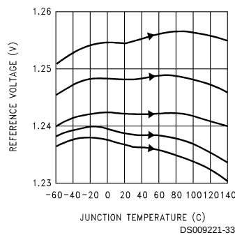
Reference Voltage vs Temp on 5 Representative Units
