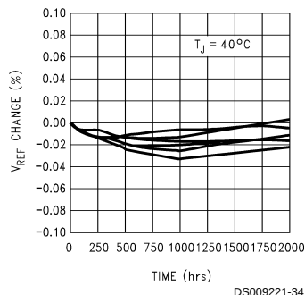
Reference Voltage Drift
