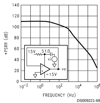
Positive Power Supply Voltage Rejection Ratio
