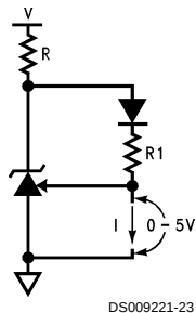
FIGURE 10. Proportional-to-Absolute-Temperature Current Source
