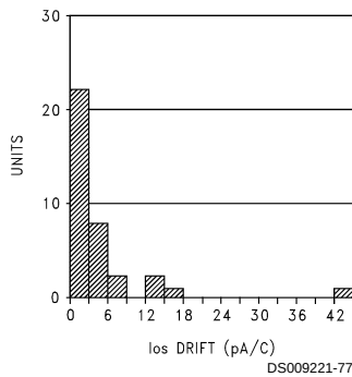
Average I_{OS} Drift Military Temperature Range
