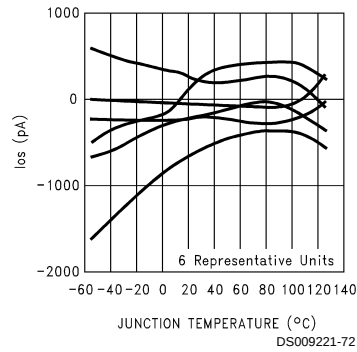
Input Offset Current vs Junction Temperature
