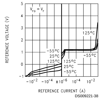
Reference Voltage vs Reference Current
