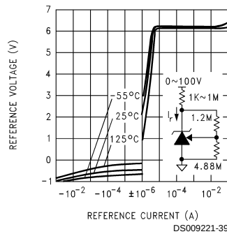
Reference Voltage vs Reference Current
