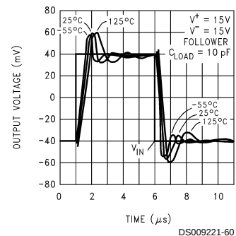
Small Signal Pulse Response vs Temp.
