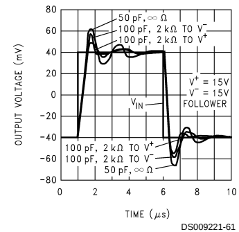
Small-Signal Pulse Response vs Load
