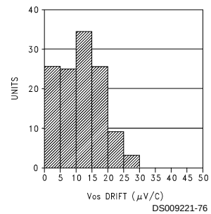
Average V_{OS} Drift Commercial Temperature Range
