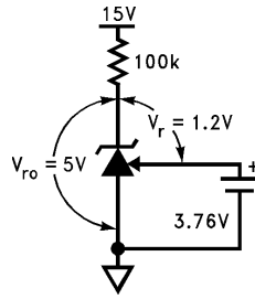
FIGURE 4. Thevenin Equivalent of Reference with 5V Output
