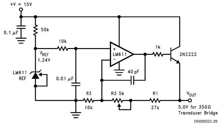
FIGURE 14. Slow Rise-Time Upon Power-Up, Adjustable Transducer Bridge Driver. Rise-time is approximately 0.5 ms.
