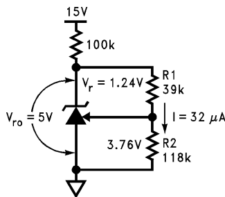
FIGURE 4. Thevenin Equivalent of Reference with 5V Output
