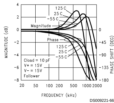
Follower Small-Signal Frequency Response
