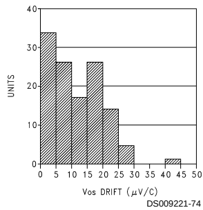
Average V_{OS} Drift Military Temperature Range
