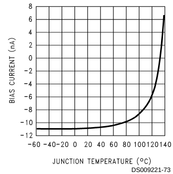
Input Bias Current vs Junction Temperature
