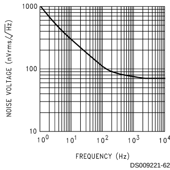
Op Amp Voltage Noise vs Frequency
