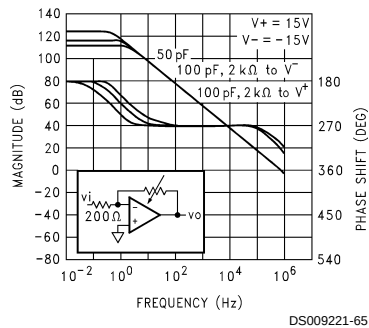
Small-Signal Voltage Gain vs Frequency and Load
