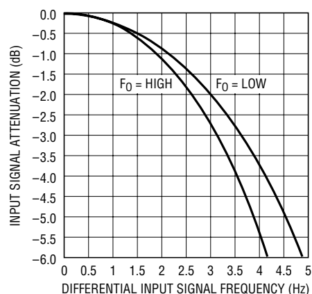
Figure 31. Input Signal Bandwidth Using the Internal Oscillator
