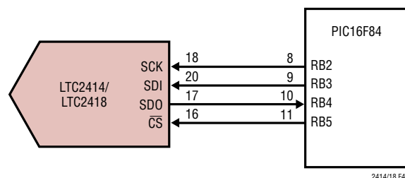
Figure 49. Connecting the LTC2414/LTC2418 to a PIC16F84 MCU Using the SPI Serial Interface
