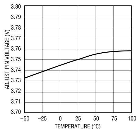
Regulator 1 Adjust Pin Voltage vs Temperature
