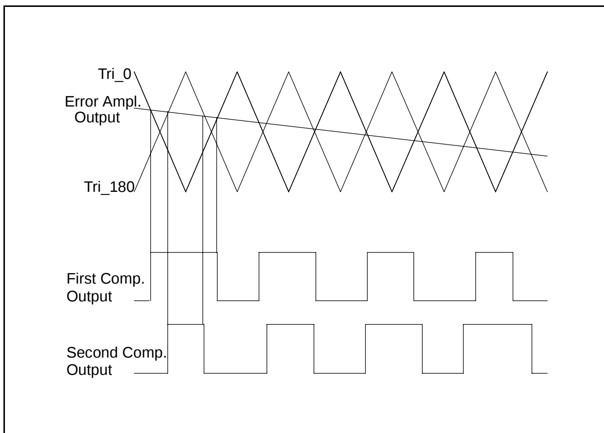
Figure 3. Output comparator waveforms
