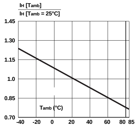
Fig. 2: Typical relative variation of holding current versus ambient temperature.
