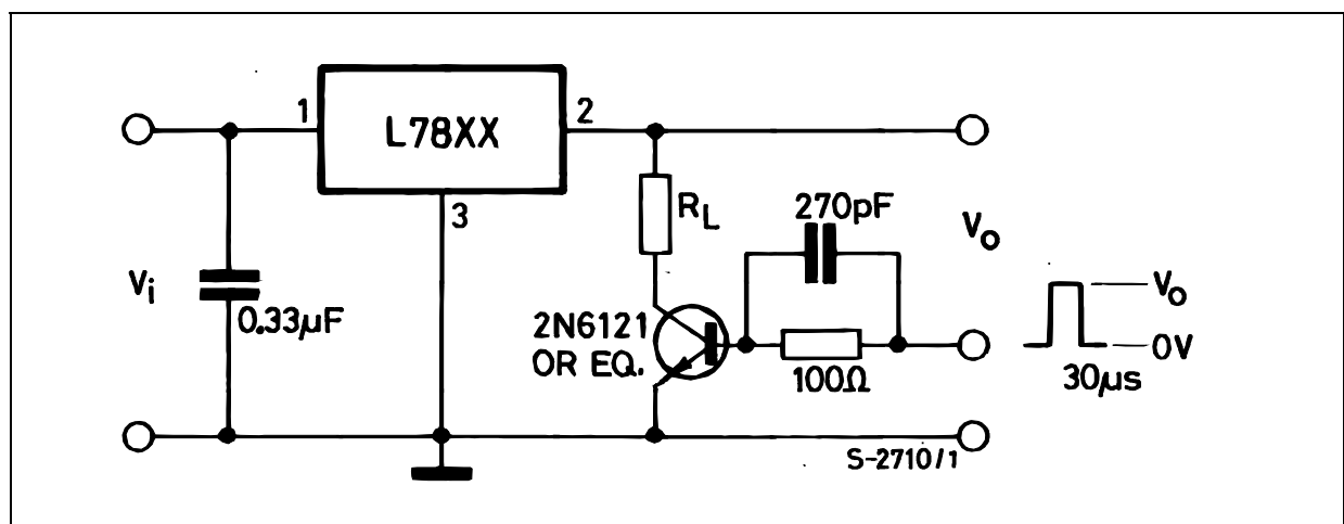
Figure 2 : Load Regulation
