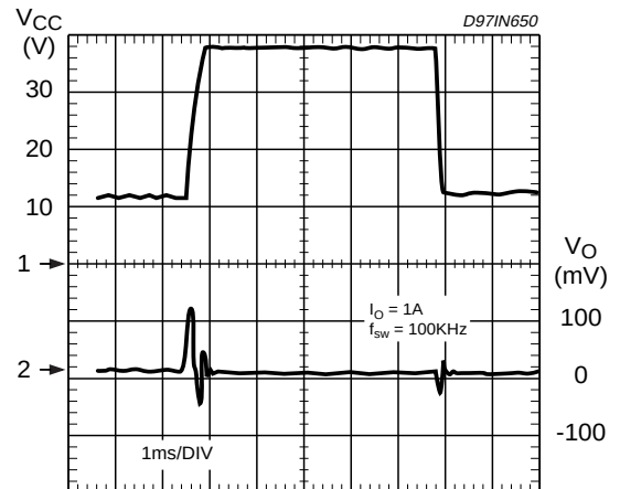
Figure 27: Line Transient
