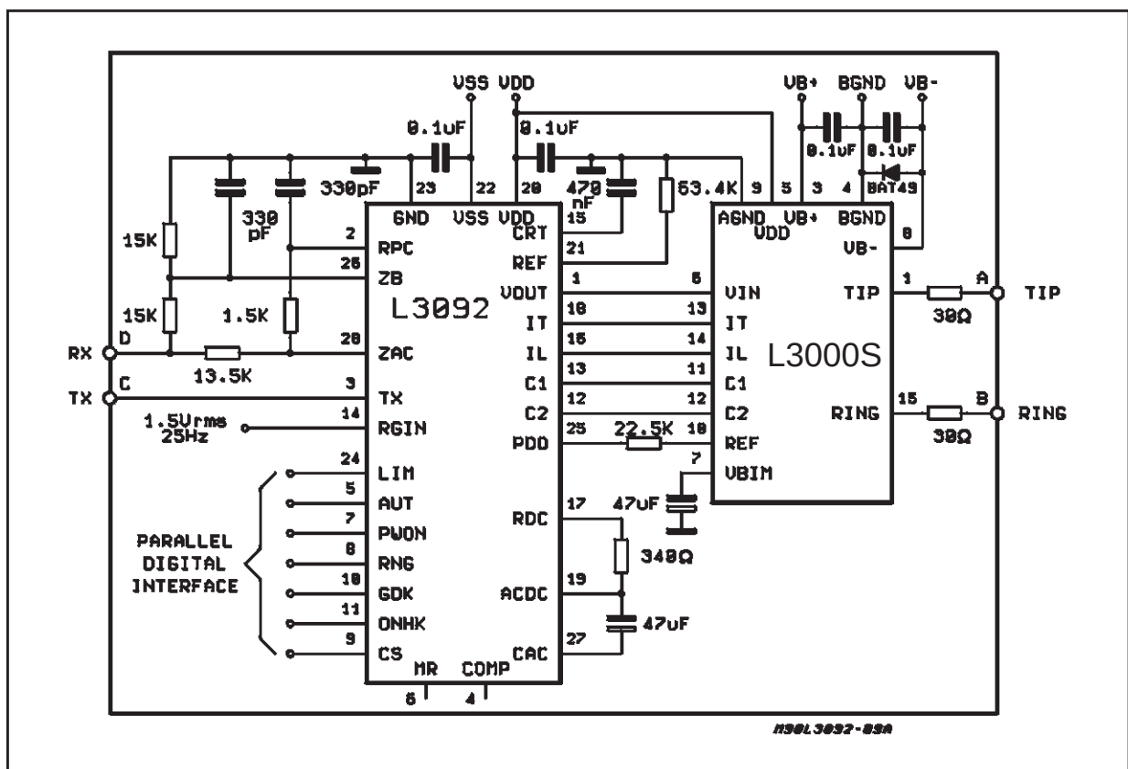
Figure 10: Test Circuit
