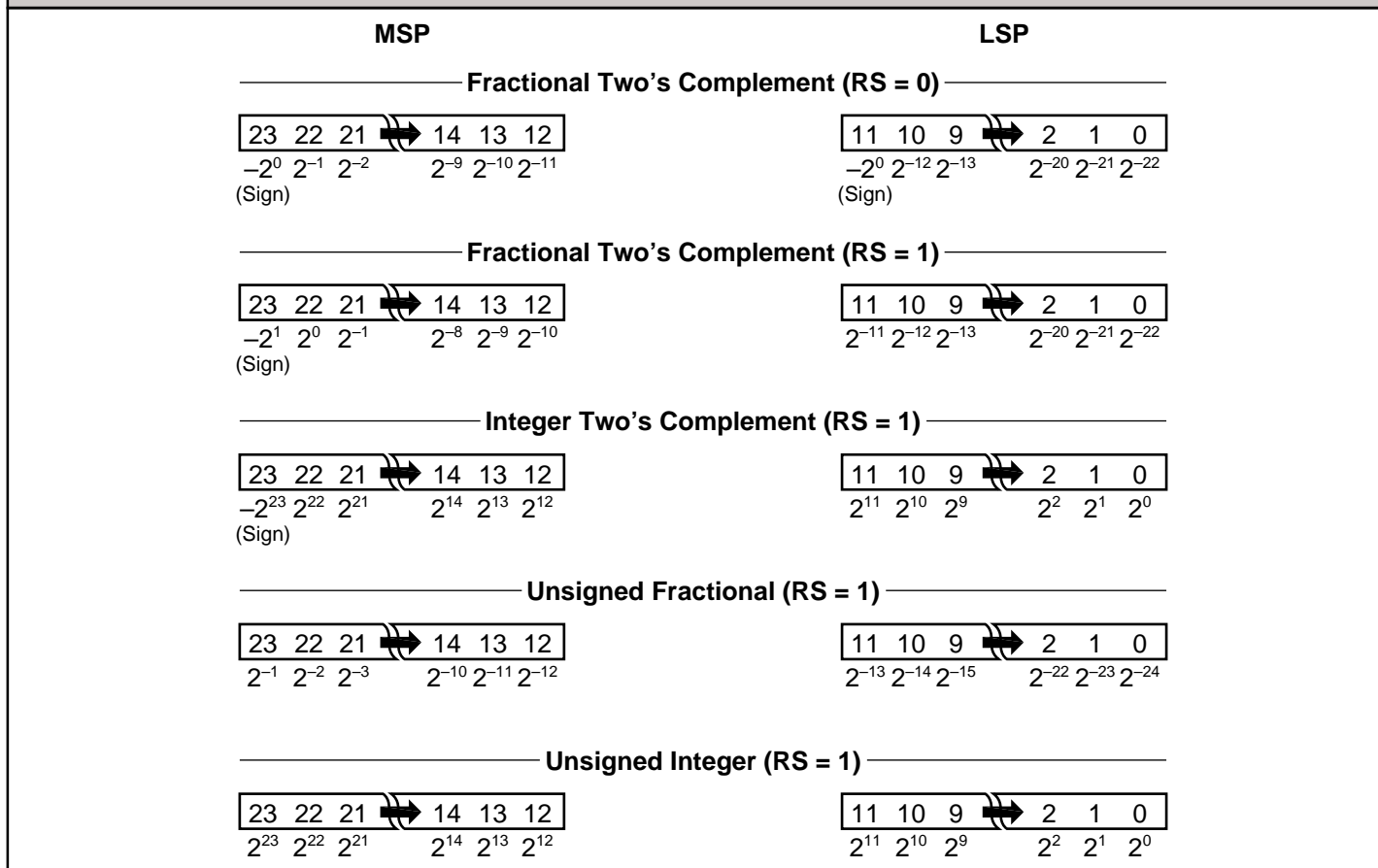
FIGURE 1B. OUTPUT FORMATS
