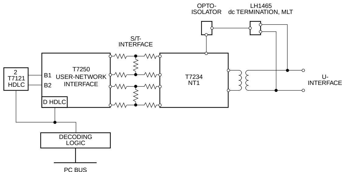
Figure 2. LH1465 Application: Passive ISDN Terminal Adapter
