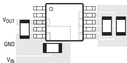
Figure 6. Recommended Layout
