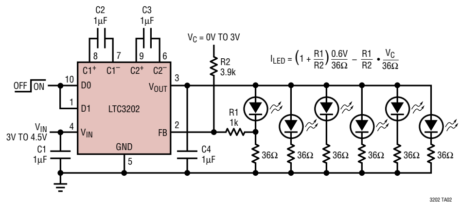
LED Driver with Linear Brightness Control
