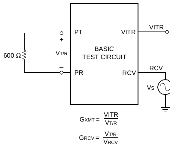
Figure 11. ac Gains
