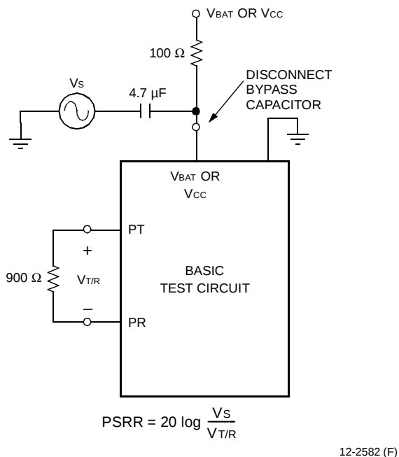
Figure 7. Metallic PSRR
