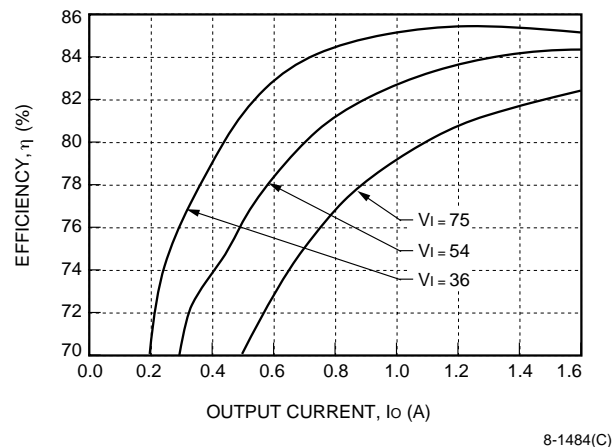
Figure 4. LW020B Typical Converter Efficiency vs. Output Current, T_A = 25^\circ\text{C}
