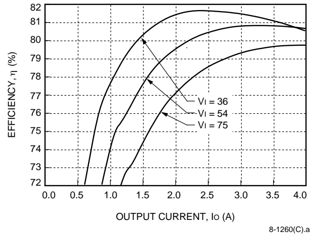
Figure 3. LW020A Typical Converter Efficiency vs. Output Current
