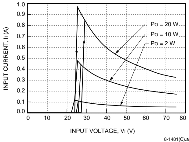
Figure 1. LW020 Typical Input Characteristics, T_A = 25^\circ\text{C}
