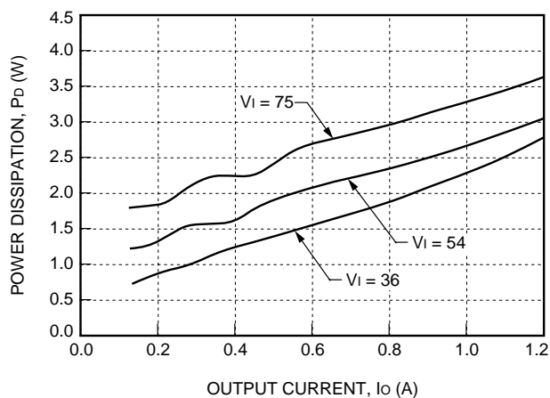
Figure 19. LW020C Power Dissipation vs. Output Current, T_A = 25^\circ\text{C}
