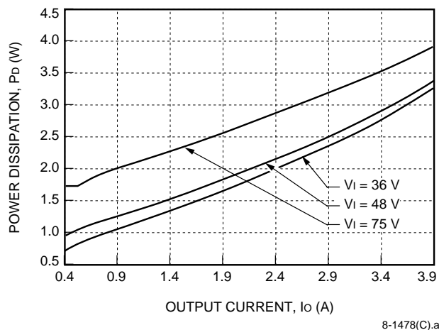
Figure 20. LW020F and G Power Dissipation vs. Output Current, T_A = 25^\circ\text{C}
