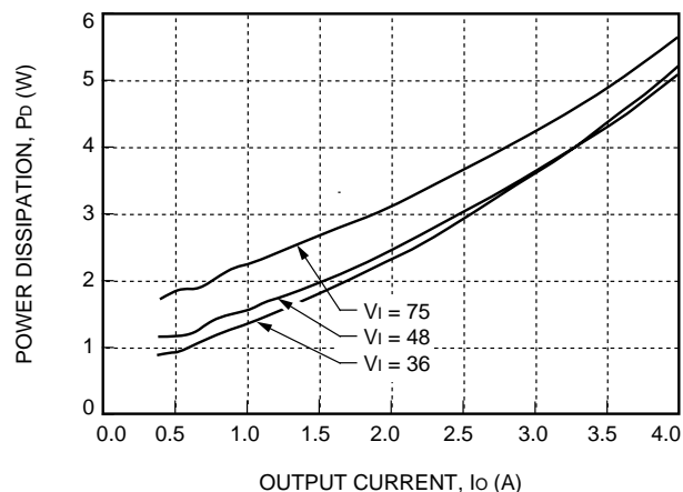
Figure 17. LW020A Power Dissipation vs. Output Current
