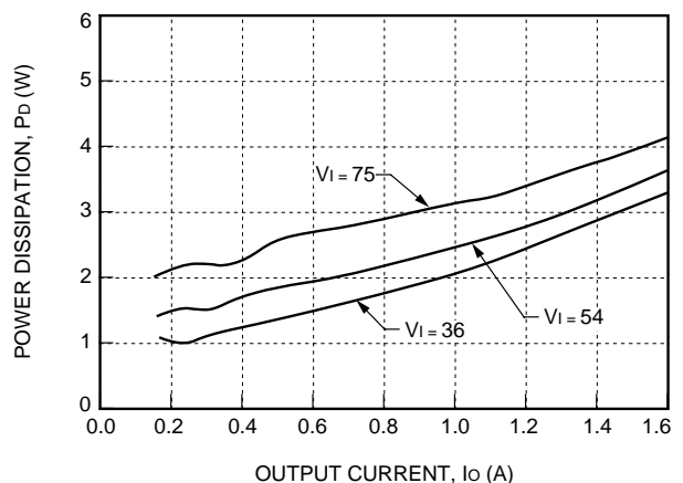
Figure 18. LW020B Power Dissipation vs. Output Current, T_A = 25^\circ\text{C}
