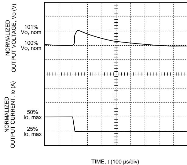
Figure 9. LW020A, B, C, F, and G Typical Output Voltage for a Step Load Change from 50% to 25%
