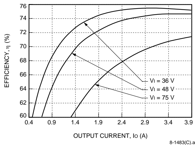
Figure 7. LW020G Typical Converter Efficiency vs. Output Current, T_A = 25^\circ\text{C}
