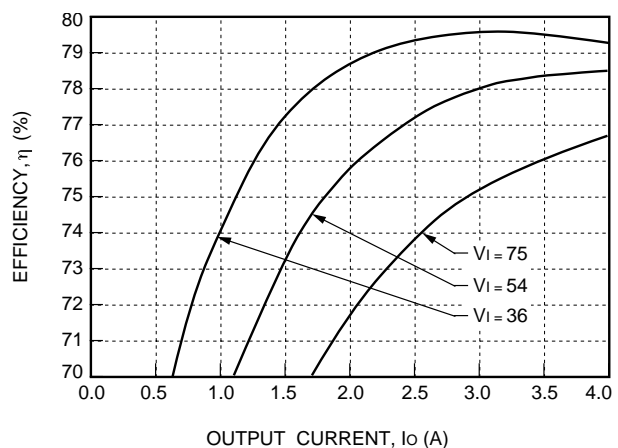
Figure 6. LW020F Typical Converter Efficiency vs. Output Current, T_A = 25^\circ\text{C}
