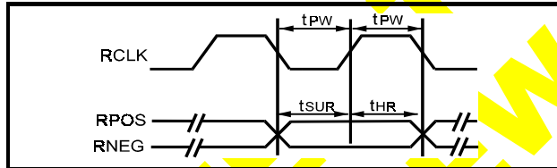
Figure 4: Clock Timing Diagram
