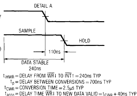
Figure 5. Timing Diagram
