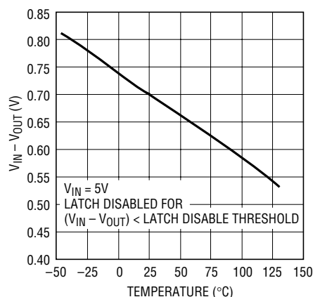
Latch-Disable Threshold ( V_{IN} - V_{OUT} ) vs Temperature
