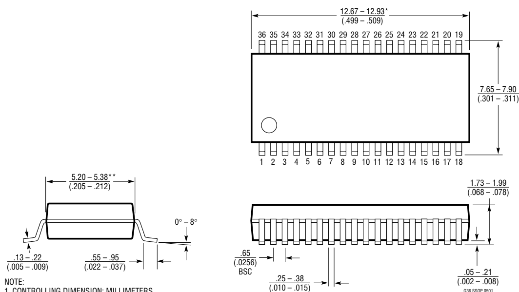
G Package 36-Lead Plastic SSOP (5.3mm) (Reference LTC DWG # 05-08-1640)
