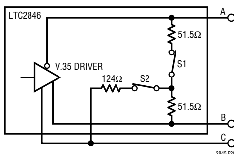
Figure 20. V.35 Driver
