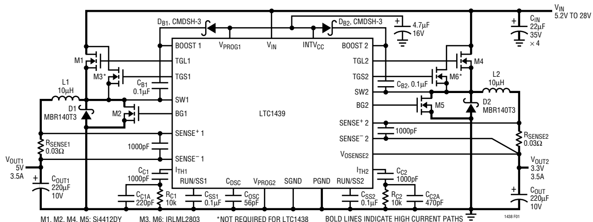
Figure 1. High Efficiency Dual 5V/3V Step-Down Converter
