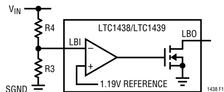
Figure 10. Low-Battery Comparator
