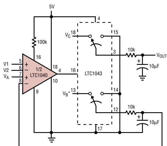
Analog Multiplier/Divider
