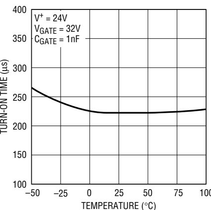
Turn-On Time vs Temperature
