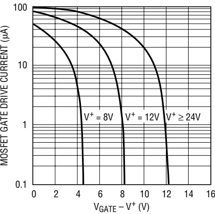
MOSFET Gate Drive Current vs V_{GATE} - V^+
