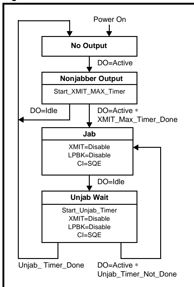
Figure 5: Jabber Control Function
