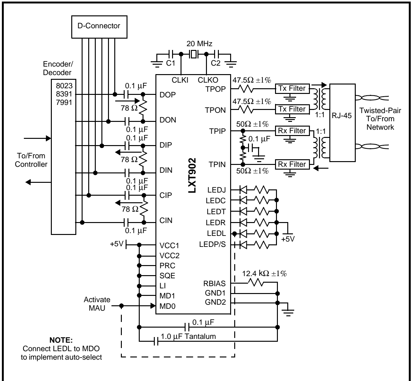
Figure 10: Typical Internal MAU Application
