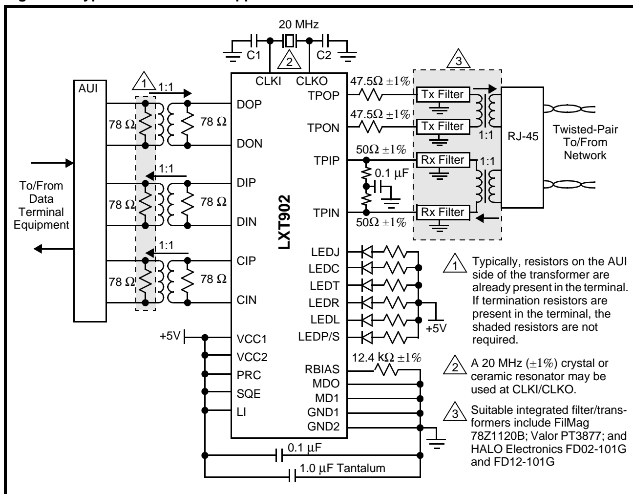
Figure 7: Typical External MAU Application
