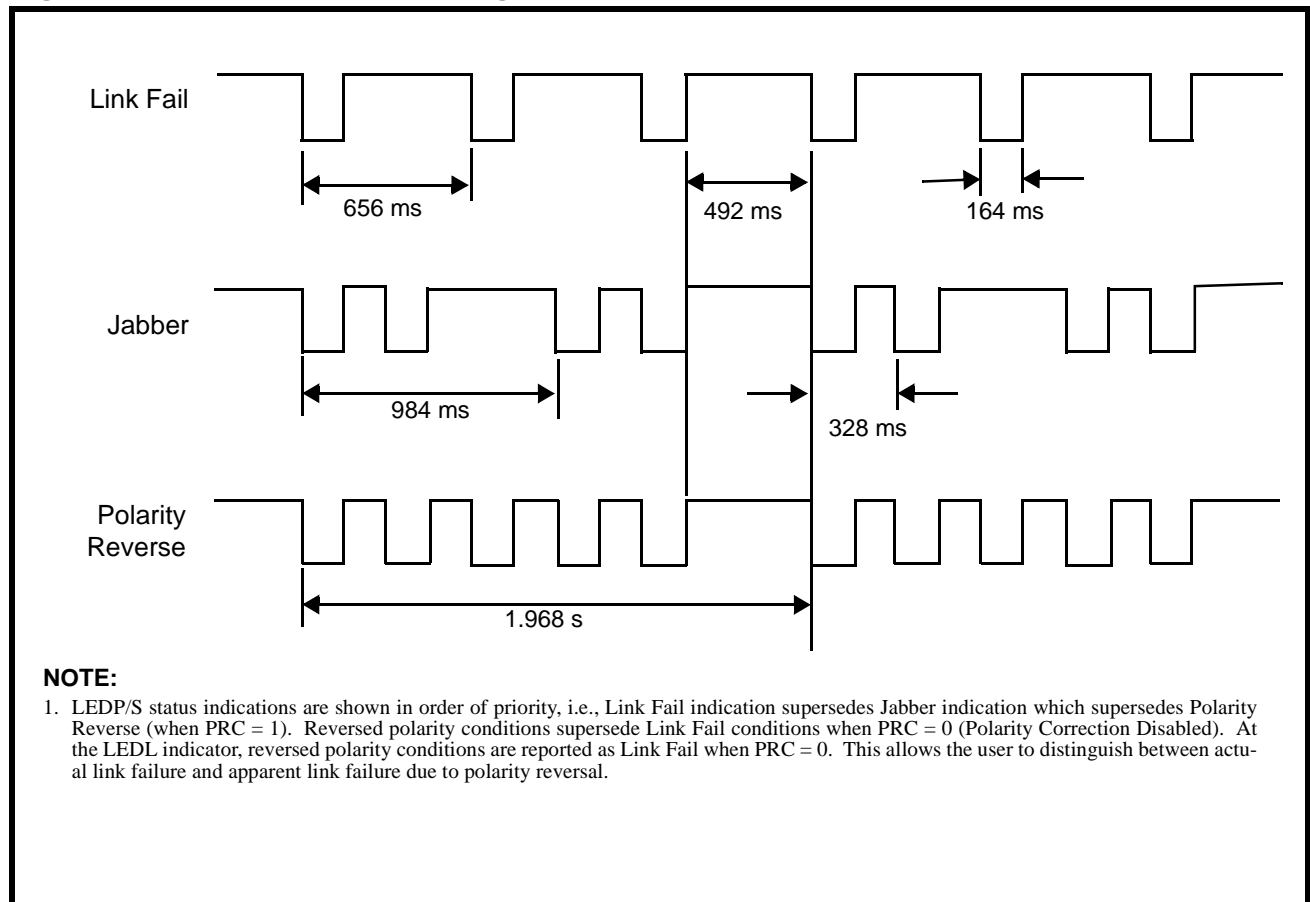
Figure 11: LEDP/S Indication Timing
