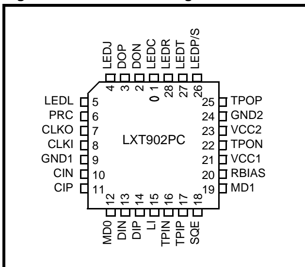
Figure 1: LXT902 Pin Assignments
