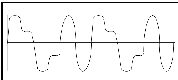
Figure 2: LXT902 TPO Output Waveform
