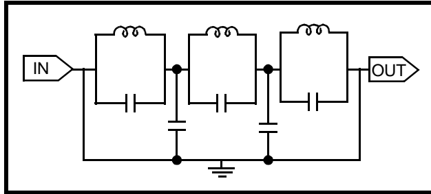
Figure 8: Typical Transmit Filter
